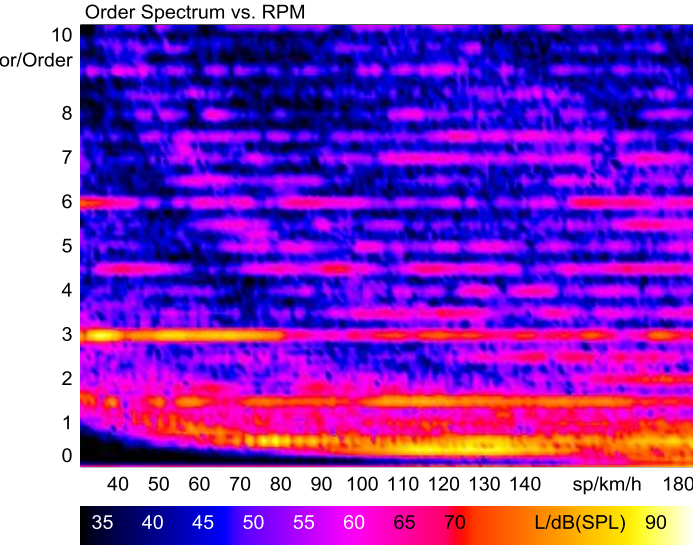
Figure 5: Order analysis calculated against engine speed and displayed versus vehicle speed
