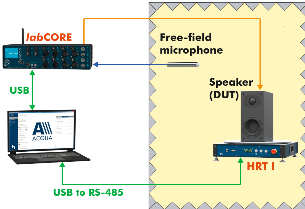
Measurement configuration for enclosed loudspeaker (exemplary)
